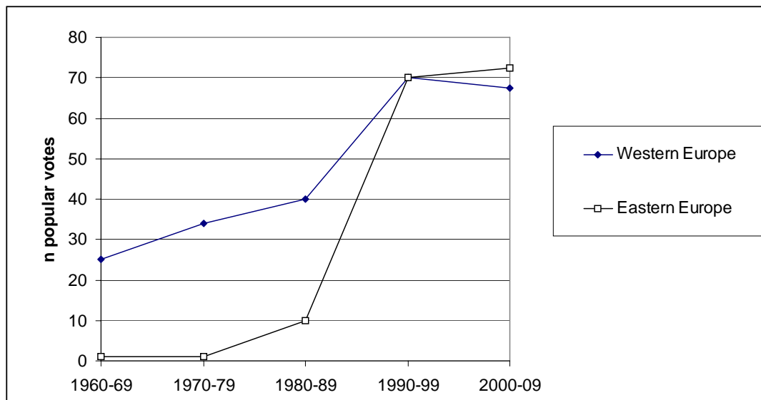
Figure 7: Overall tendency of direct democratic votes in Western and Eastern and Central Europe (all Council of Europe countries without Switzerland)
