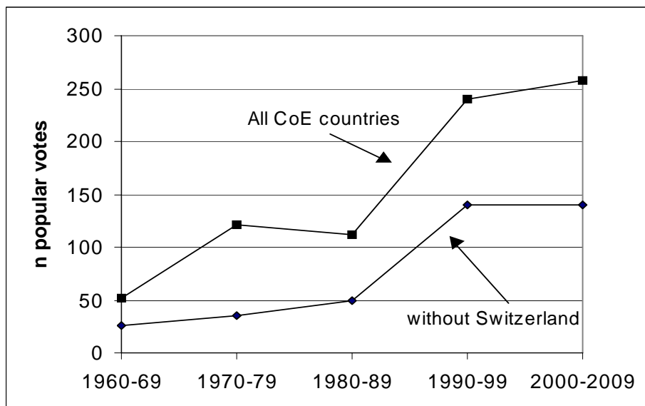
Figure 6: Overall tendency of direct democratic votes in all Council of Europe countries and with Switzerland excluded
